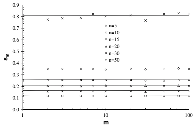
Fig. 5 The effect of m and n on s_m for the maximum likelihood method
